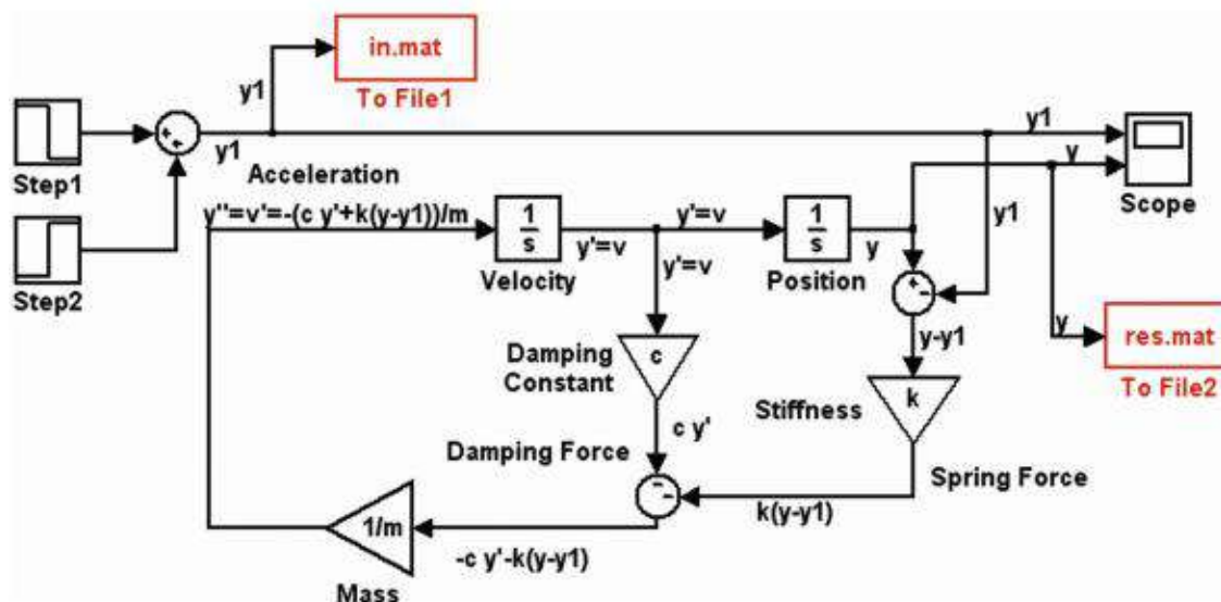
1.12 – rasm. Avtomobilning ko'tarib turuvchi tzizmining matematik modeli
