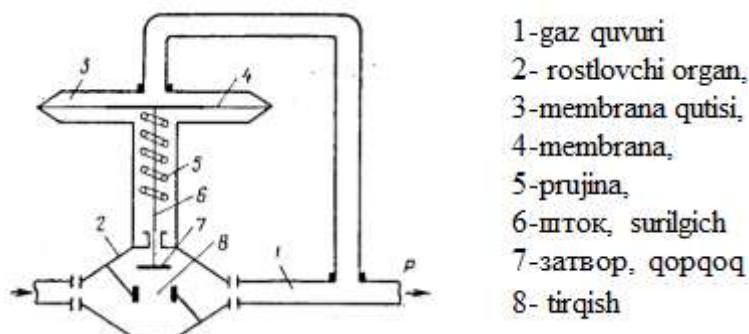
1.1-rasm. Gaz bosimini stabillashtiruvchi P rostlagich.
