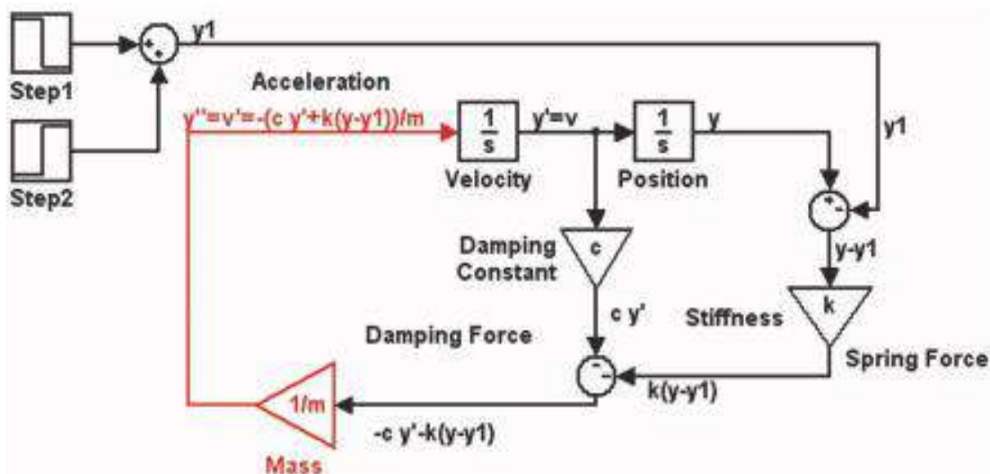
1.11 – rasm. Avtomobil harakatini hisoblash uchun toliq sistema
