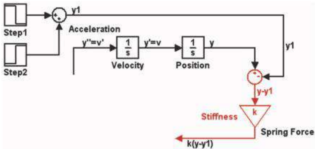
1.9 – rasm. Prujinanig bikirligi hisobga olingan modeli
