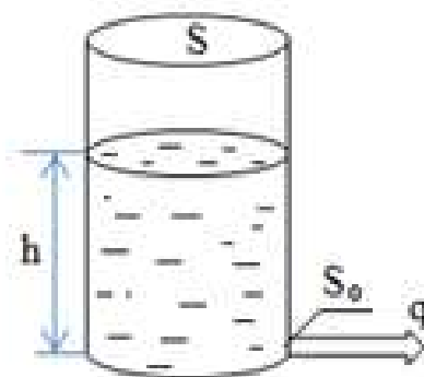
1.3-rasm. Jo'mrakli idish
