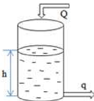
1.4-rasm. Sathni boshqarish masalasi
